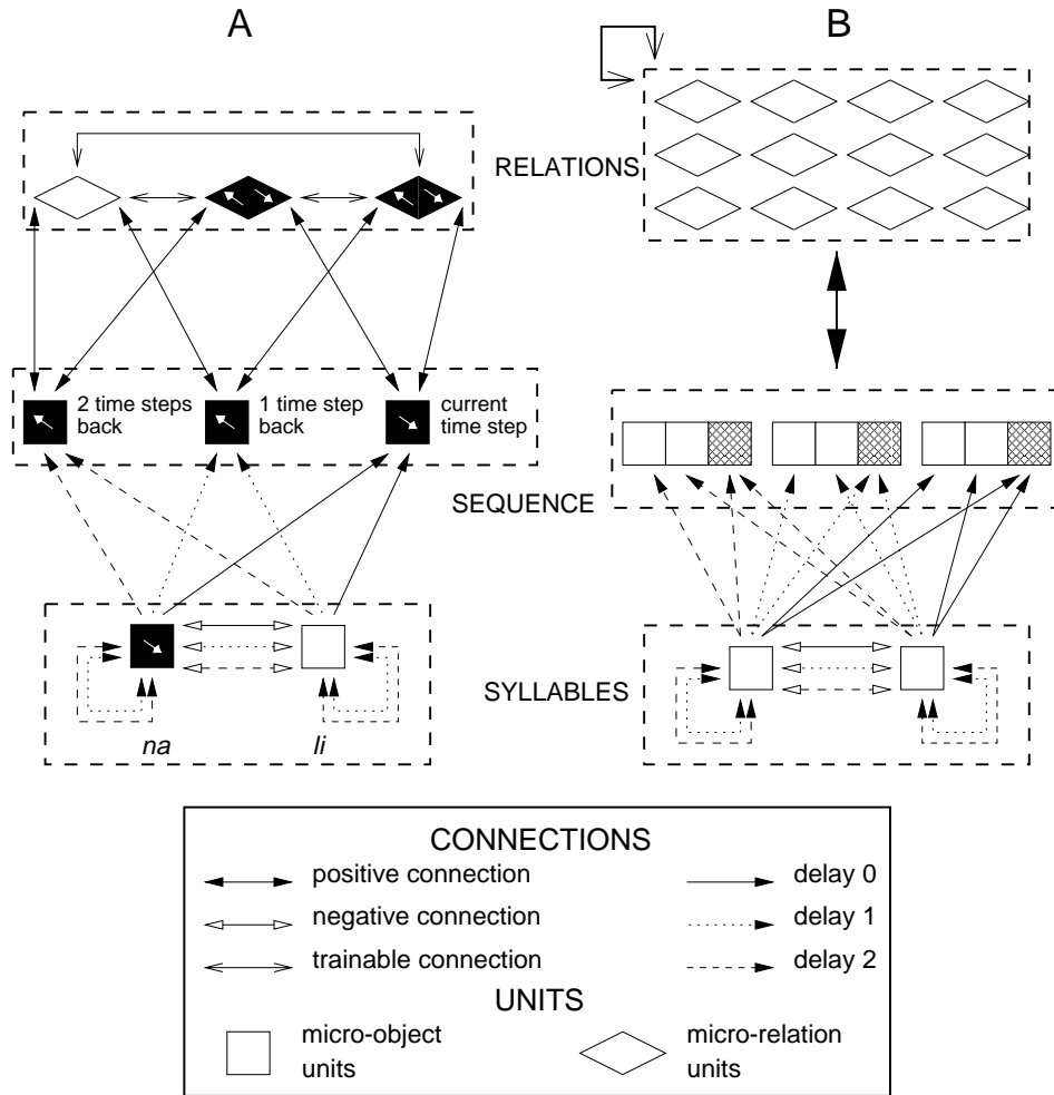
Figure 2. PLAYPEN networks for learning word sequences. (A) Simplified network used in the simulation of Marcus et al.'s experiments. Only two of the four Syllables units are shown, and the micro-role-to-micro-role mappings are not shown for the MRU connections. The sequence li li na has just been presented to the network. MOU and MRU phase angles are represented as arrows. (B) Full-blown version of the network, including syllable-specific, as well as content-free Sequence units (shaded squares). Not all connections are shown.
