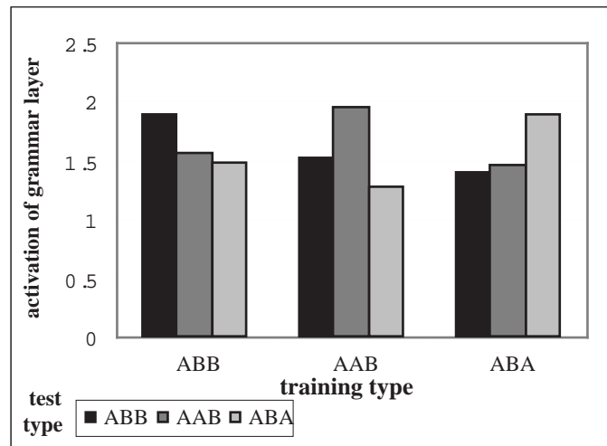
Figure 3. Networks that have been trained on sequences following a certain grammatical pattern respond with more activation to novel sequences obeying that same pattern than to novel sequences obeying other patterns.
