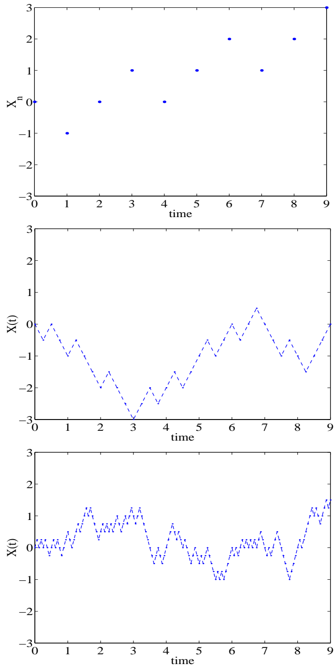
Figure 1: Sample path for the random walk with step size \Delta = 1 (top); \Delta = .5 (middle); and \Delta = .25 (bottom).
